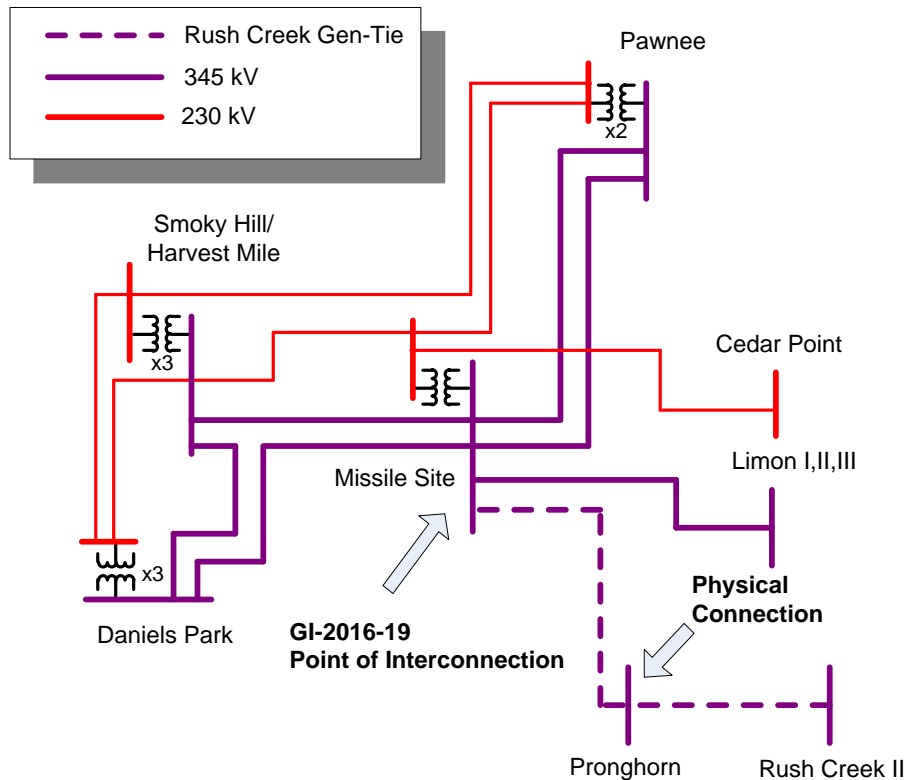
Figure 1: Conceptual one-line of proposed physical connection, the POI and surrounding Transmission System
