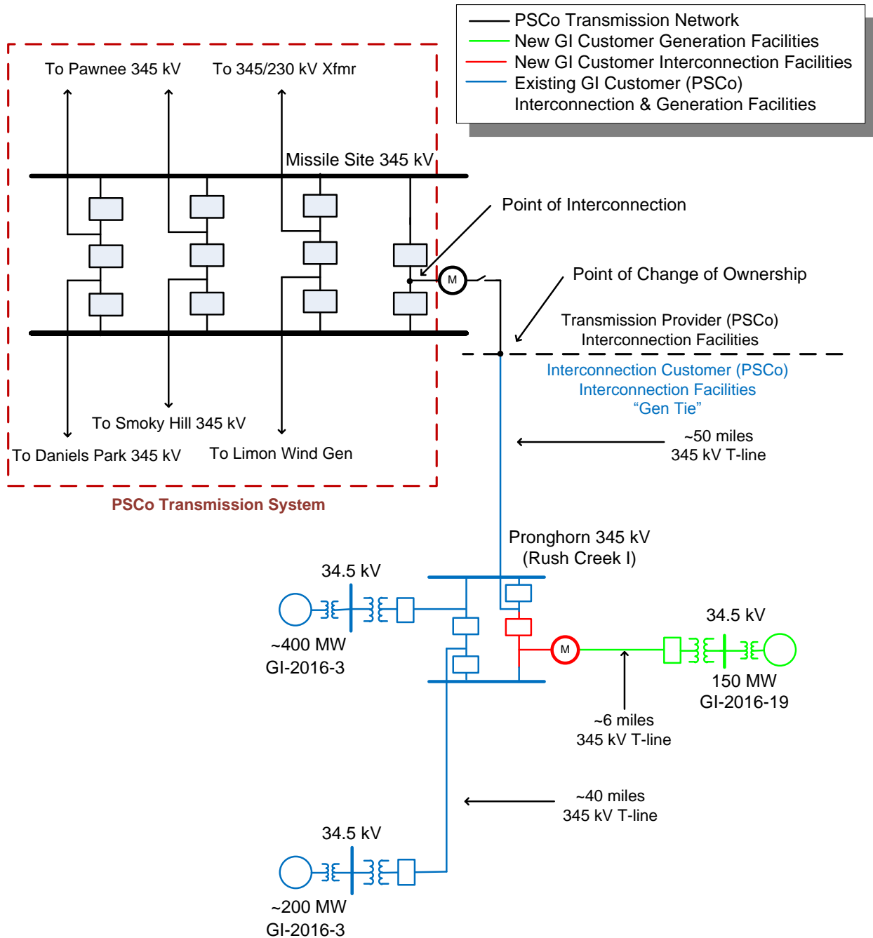
Figure 2: GI-2016-19 Interconnection to the Missile Site 345kV Bus POI via Existing Rush Creek Gen-Tie and Pronghorn Switching Station Interconnection Facilities
